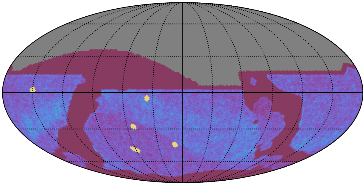
roll_pause_mjdp180_v3.4_10yrs All sky all bands: NVisits
