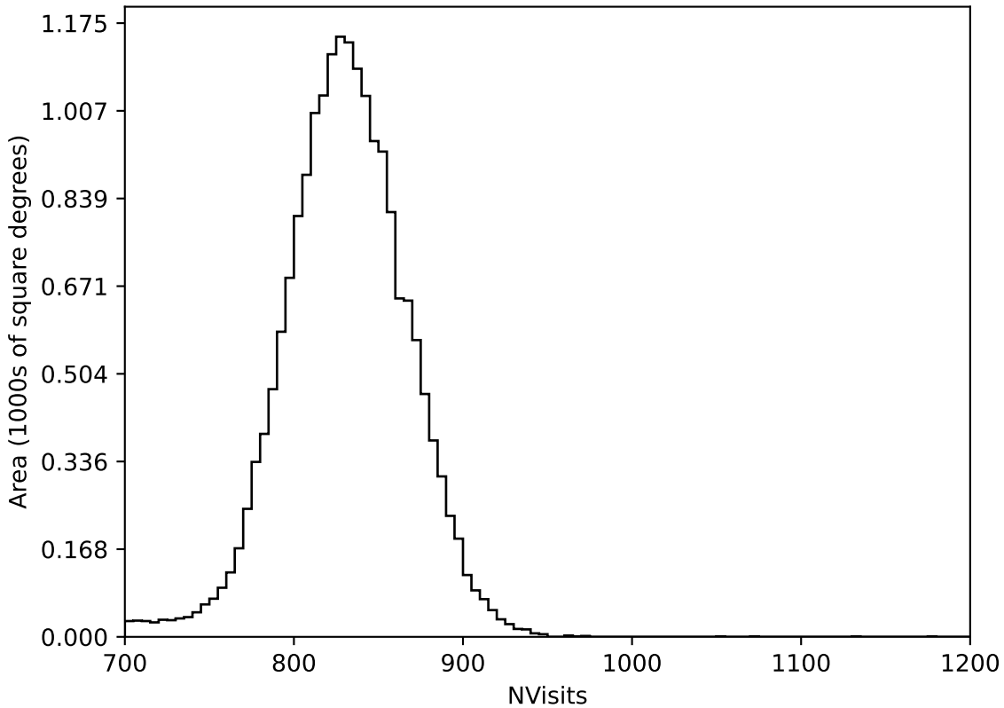
roll_pause_mjdp180_v3.4_10yrs All sky all bands: NVisits
