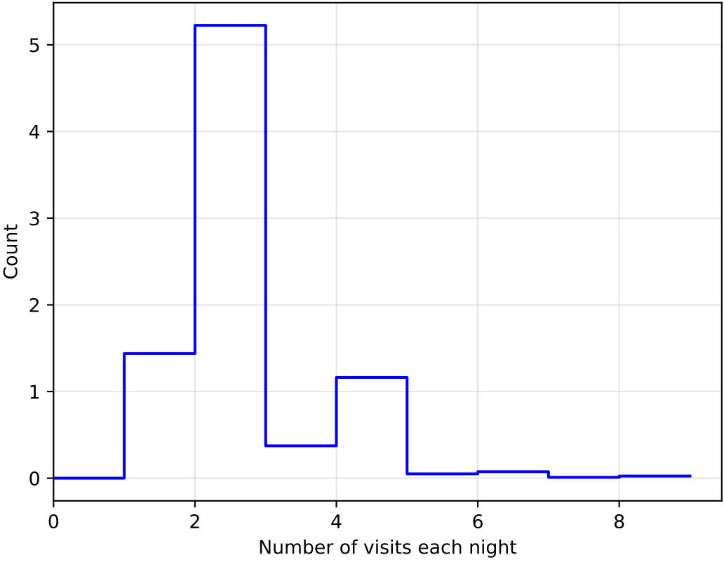
roll_pause_mjdp180_v3.4_10yrs WFD: NVisitsPerNight
