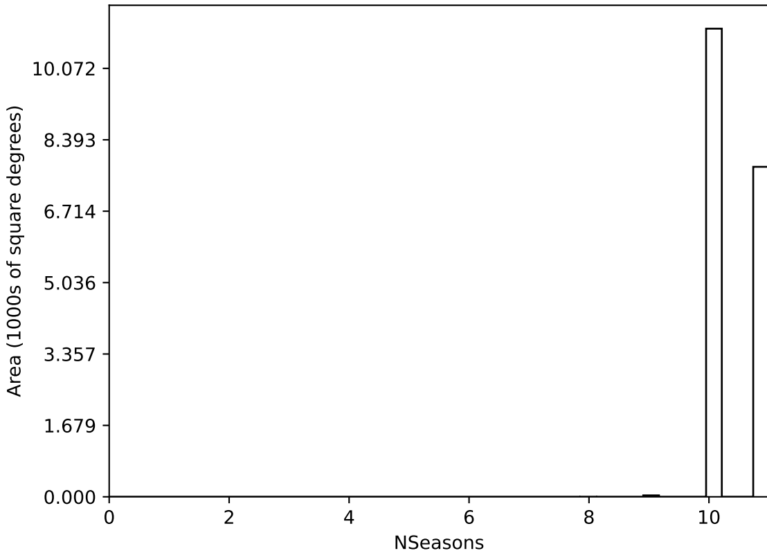
roll_pause_mjdp180_v3.4_10yrs WFD all bands: NSeasons
