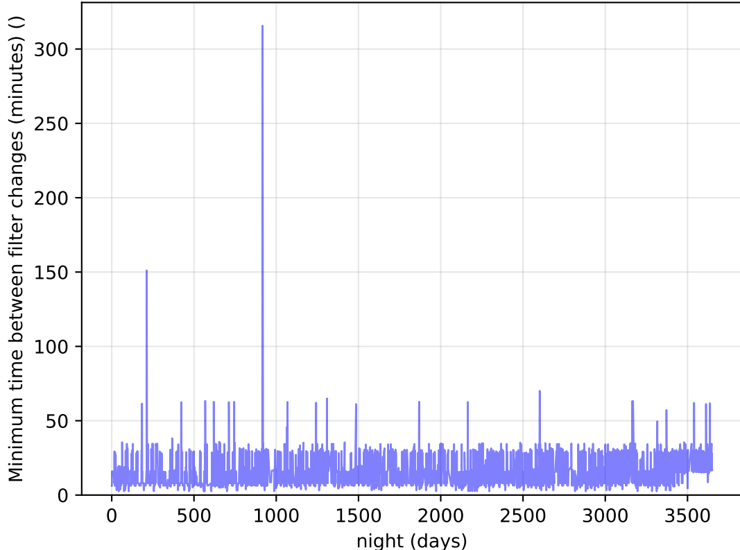
roll_pause_mjdp180_v3.4_10yrs Per Night: Minimum time between filter changes (minutes)
