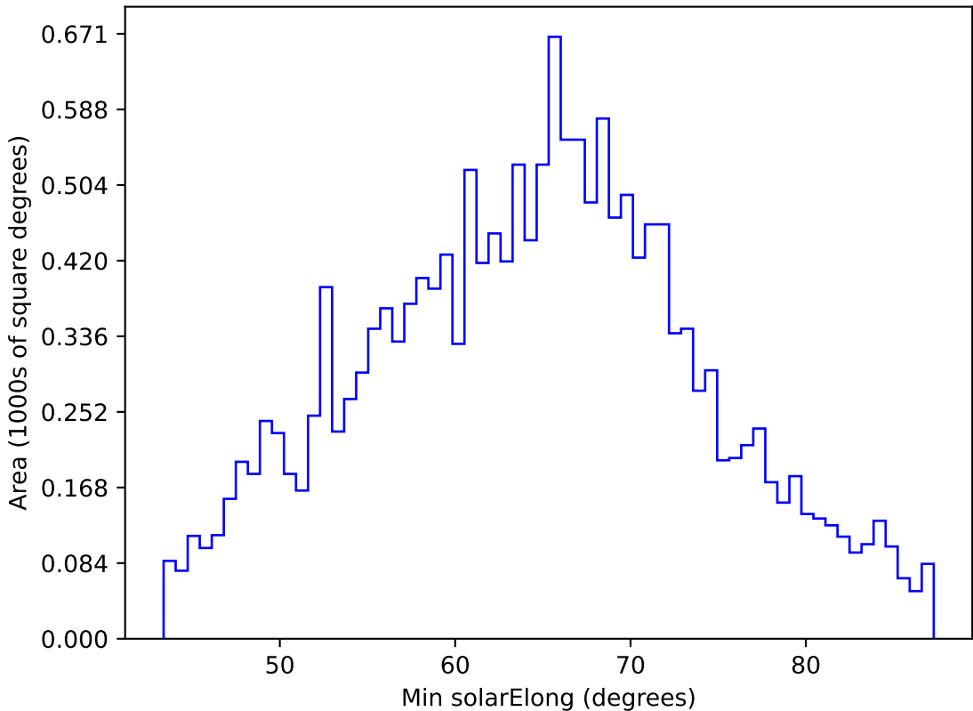
roll_pause_mjdp180_v3.4_10yrs WFD y band: Min solarElong
