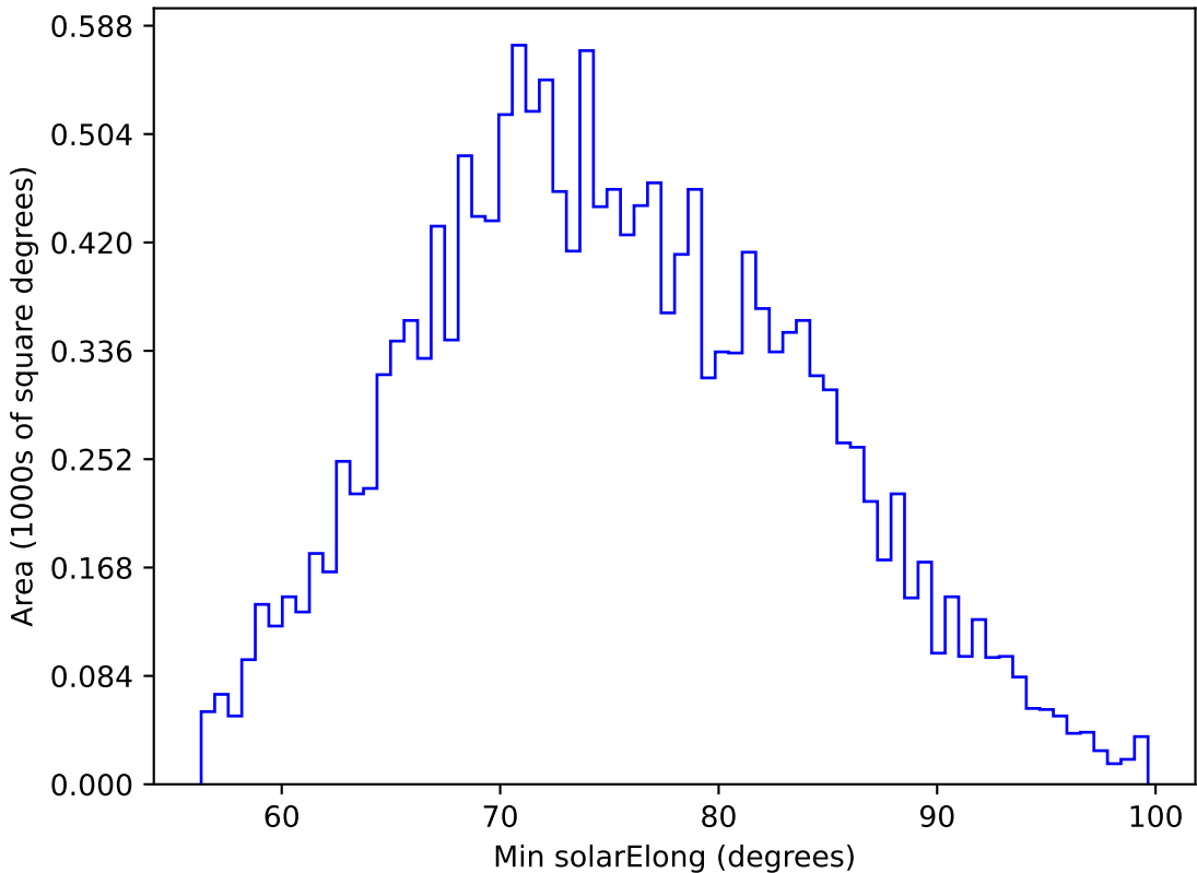
roll_pause_mjdp180_v3.4_10yrs WFD u band: Min solarElong
