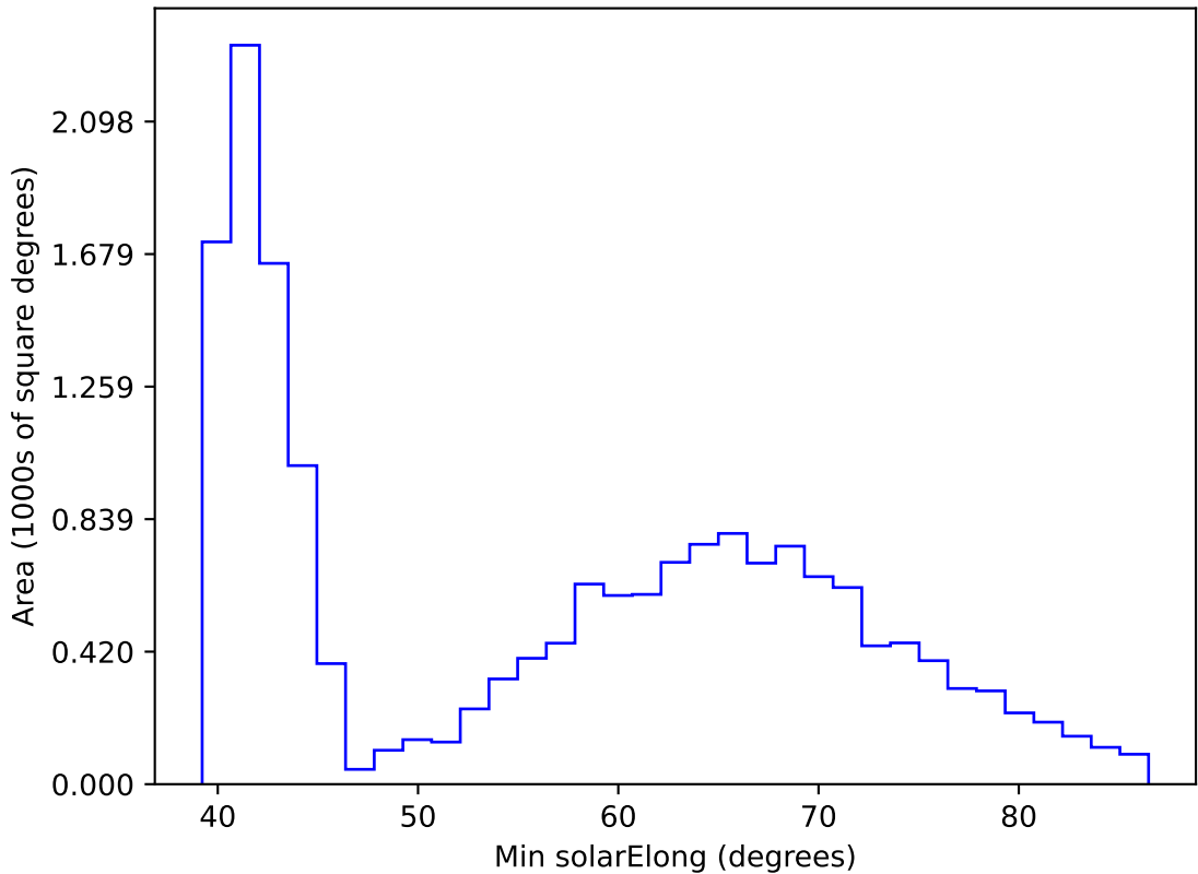
roll_pause_mjdp180_v3.4_10yrs WFD r band: Min solarElong
