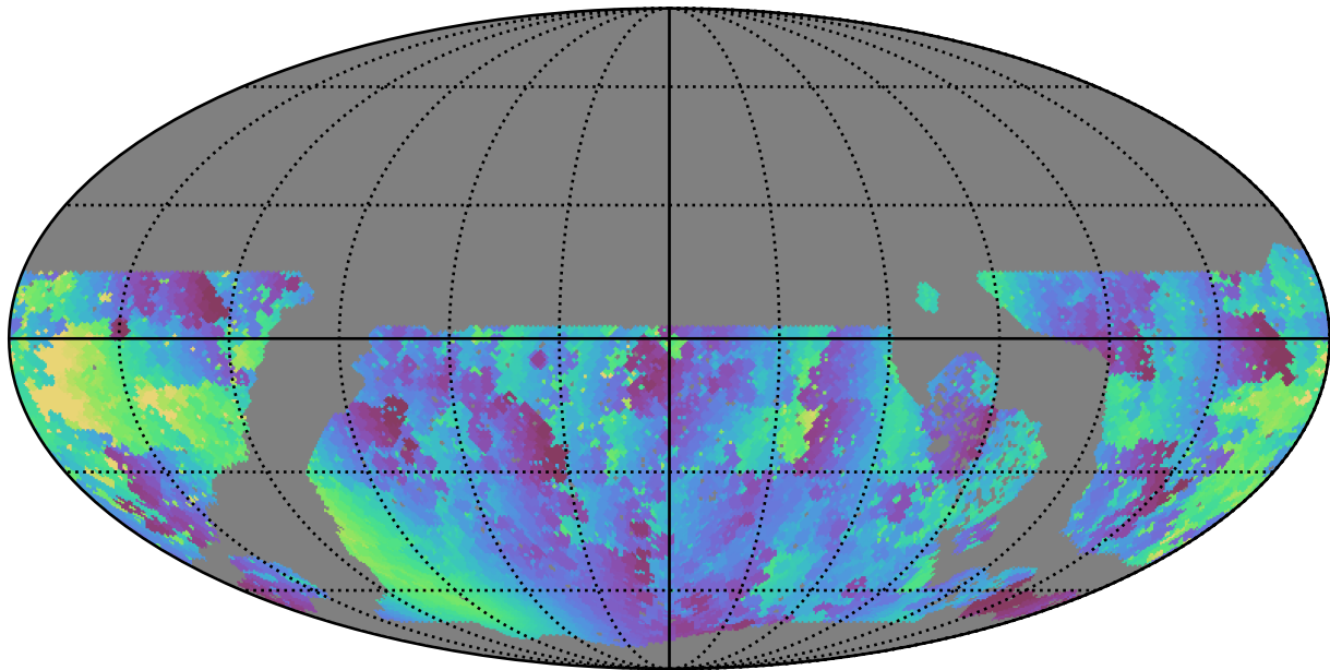
roll_pause_mjdp180_v3.4_10yrs WFD g band: Min solarElong
