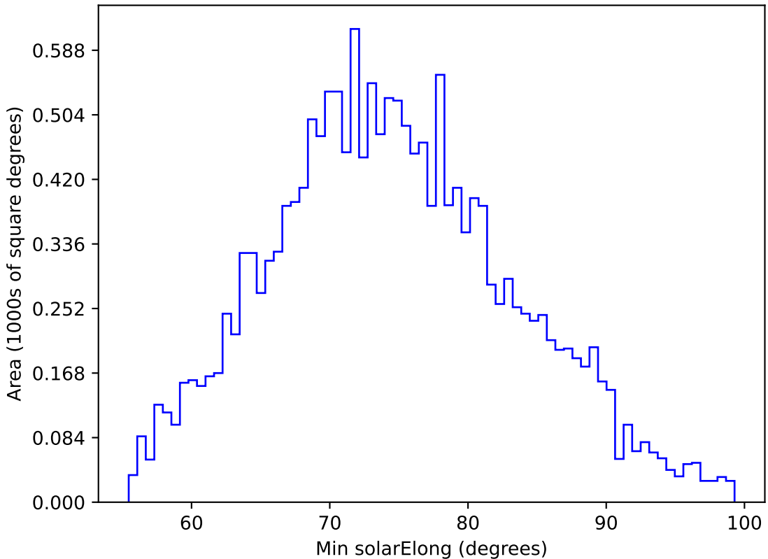
roll_pause_mjdp180_v3.4_10yrs WFD g band: Min solarElong
