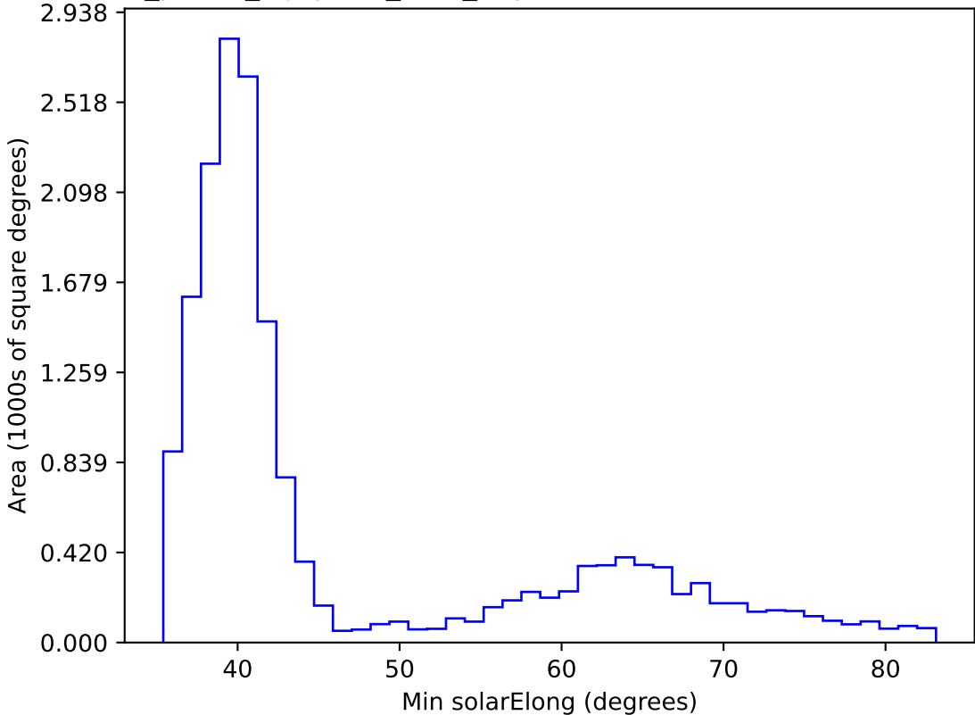
roll_pause_mjdp180_v3.4_10yrs WFD all bands: Min solarElong
