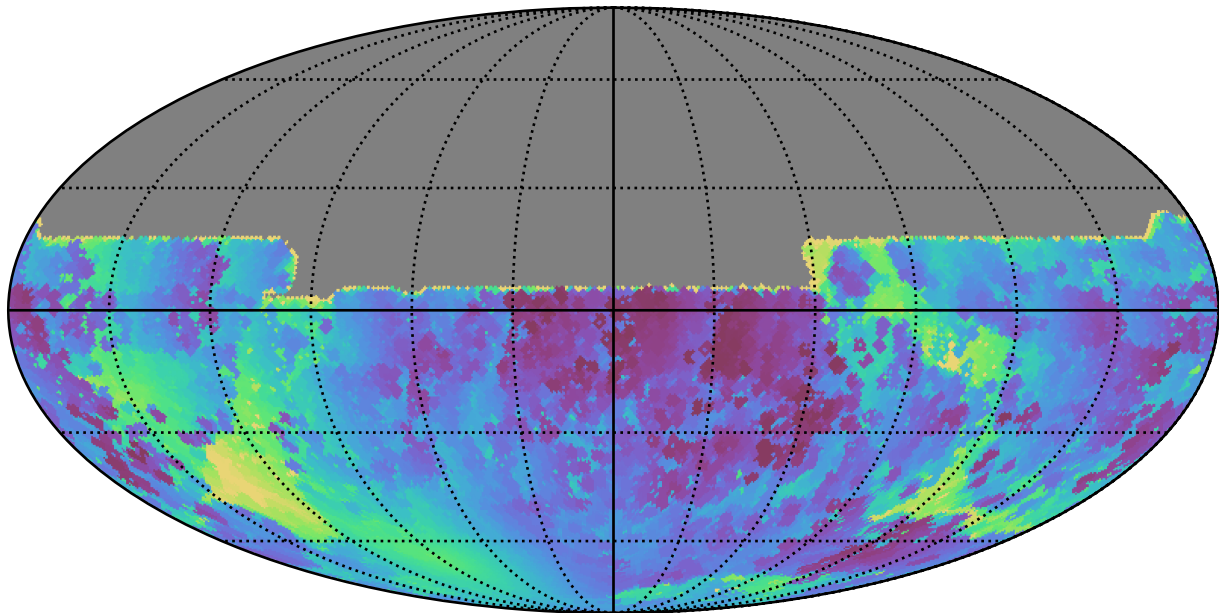
roll_pause_mjdp180_v3.4_10yrs All sky y band: Min solarElong
