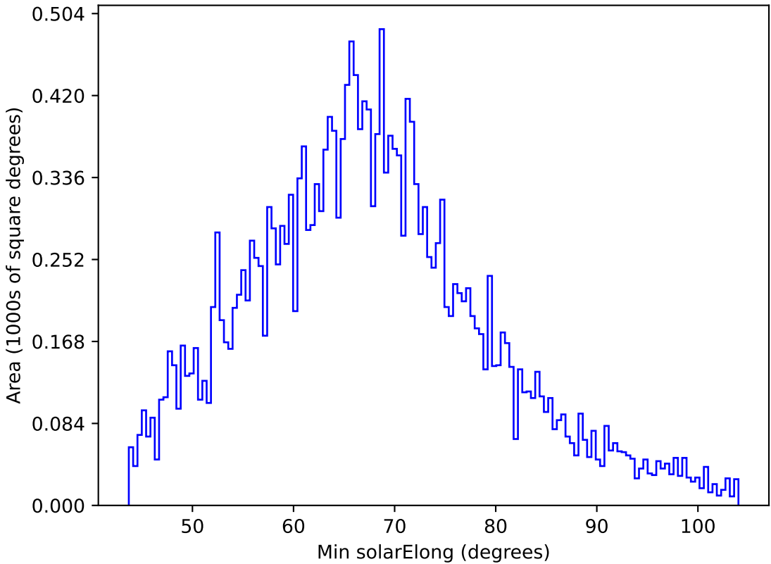
roll_pause_mjdp180_v3.4_10yrs All sky y band: Min solarElong
