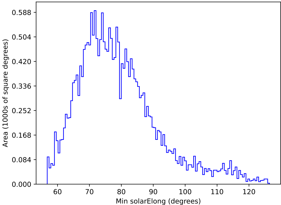
roll_pause_mjdp180_v3.4_10yrs All sky u band: Min solarElong
