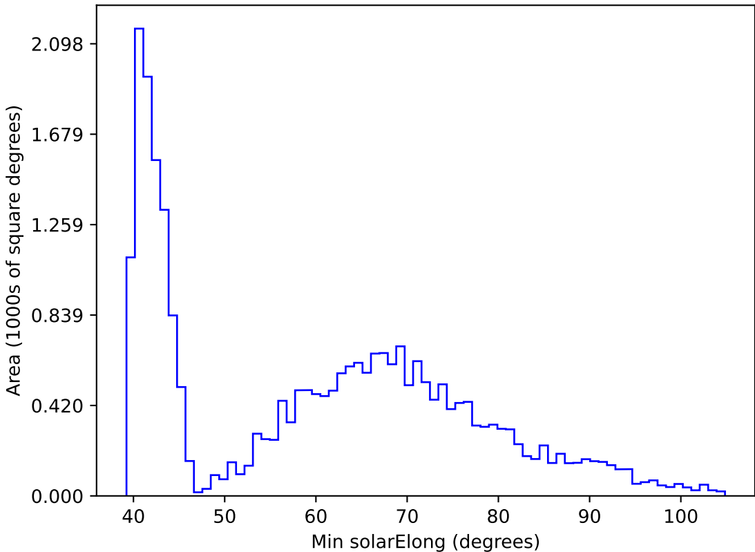
roll_pause_mjdp180_v3.4_10yrs All sky r band: Min solarElong
