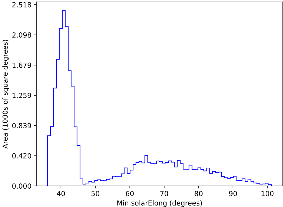
roll_pause_mjdp180_v3.4_10yrs All sky i band: Min solarElong
