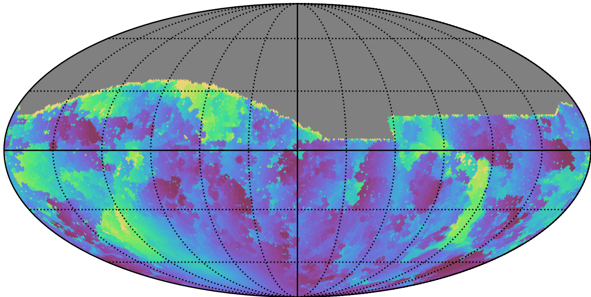
roll_pause_mjdp180_v3.4_10yrs All sky g band: Min solarElong
