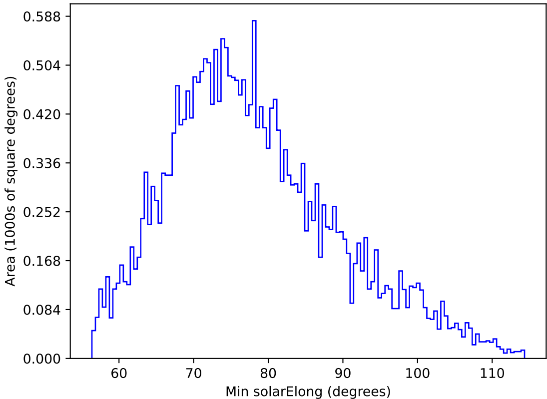
roll_pause_mjdp180_v3.4_10yrs All sky g band: Min solarElong
