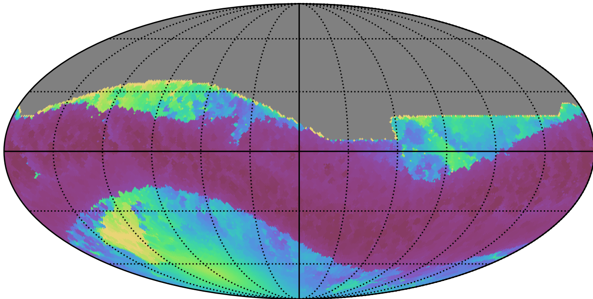
roll_pause_mjdp180_v3.4_10yrs All sky all bands: Min solarElong
