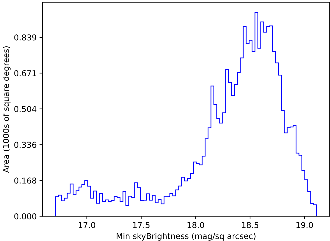
roll_pause_mjdp180_v3.4_10yrs Yr 1 z band: Min skyBrightness
