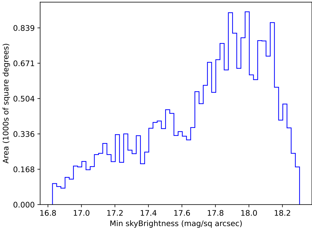
roll_pause_mjdp180_v3.4_10yrs Yr 1 y band: Min skyBrightness
