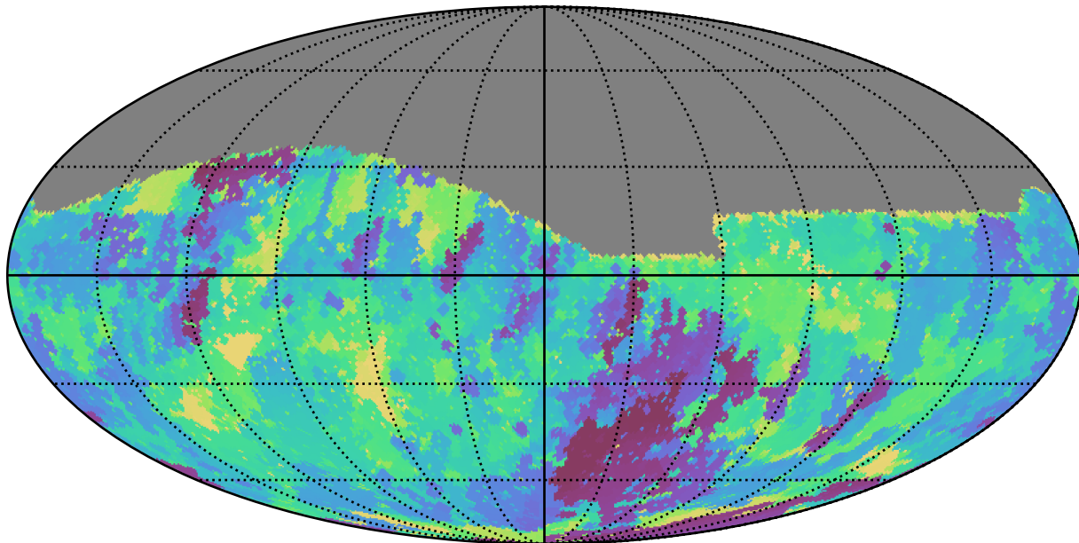
roll_pause_mjdp180_v3.4_10yrs Yr 1 r band: Min skyBrightness
