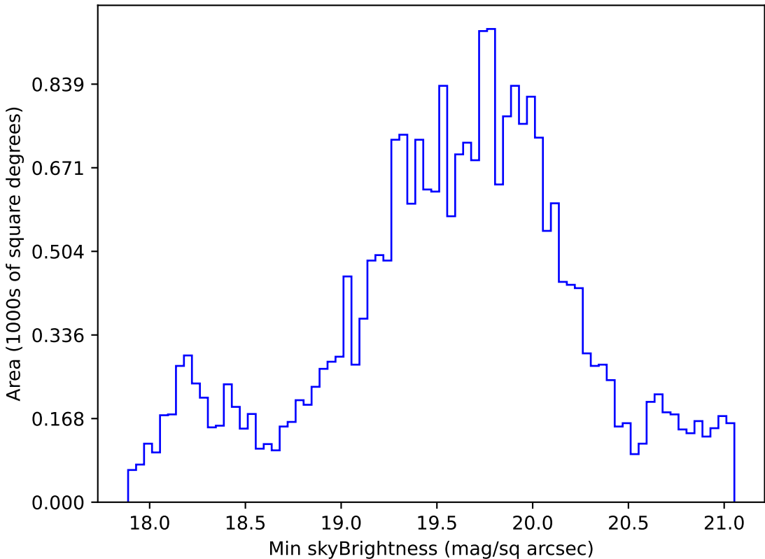
roll_pause_mjdp180_v3.4_10yrs Yr 1 r band: Min skyBrightness
