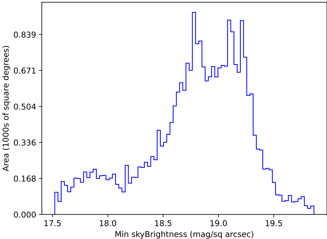
roll_pause_mjdp180_v3.4_10yrs Yr 1 i band: Min skyBrightness
