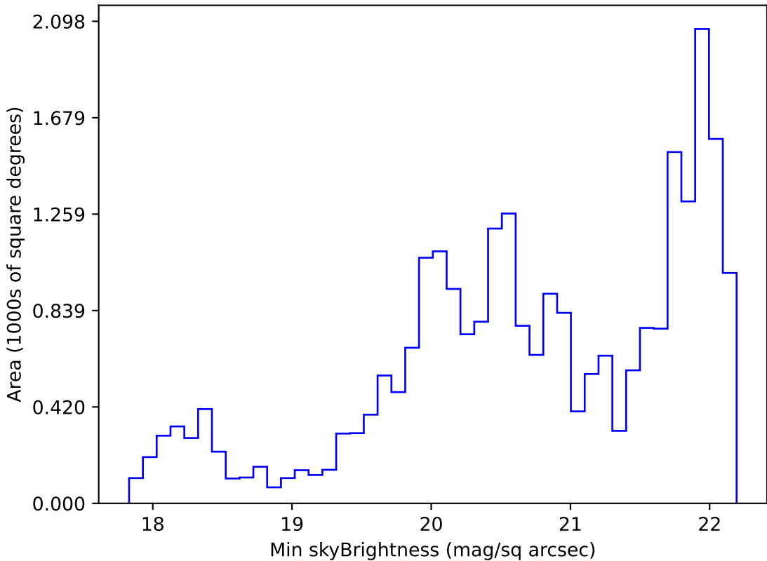
roll_pause_mjdp180_v3.4_10yrs Yr 1 g band: Min skyBrightness
