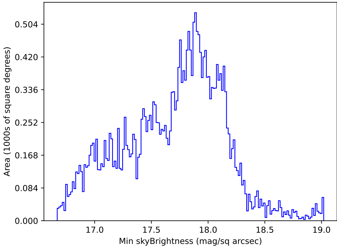
roll_pause_mjdp180_v3.4_10yrs Yr 1 all bands: Min skyBrightness
