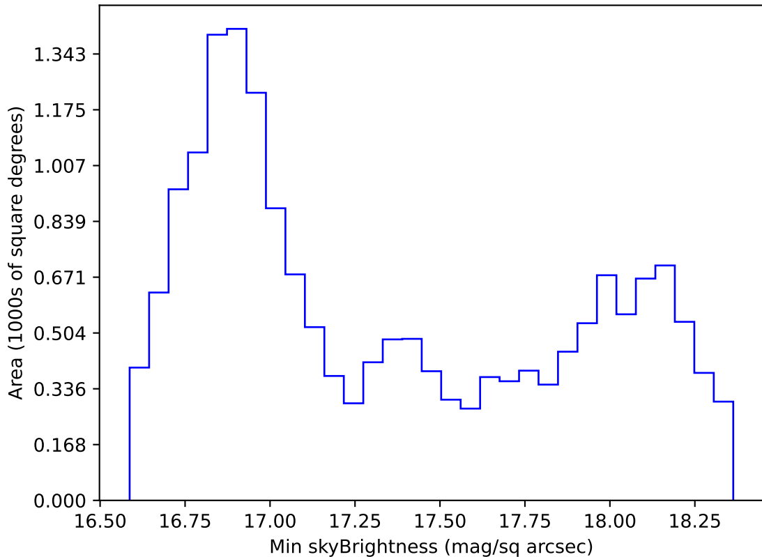
roll_pause_mjdp180_v3.4_10yrs WFD z band: Min skyBrightness
