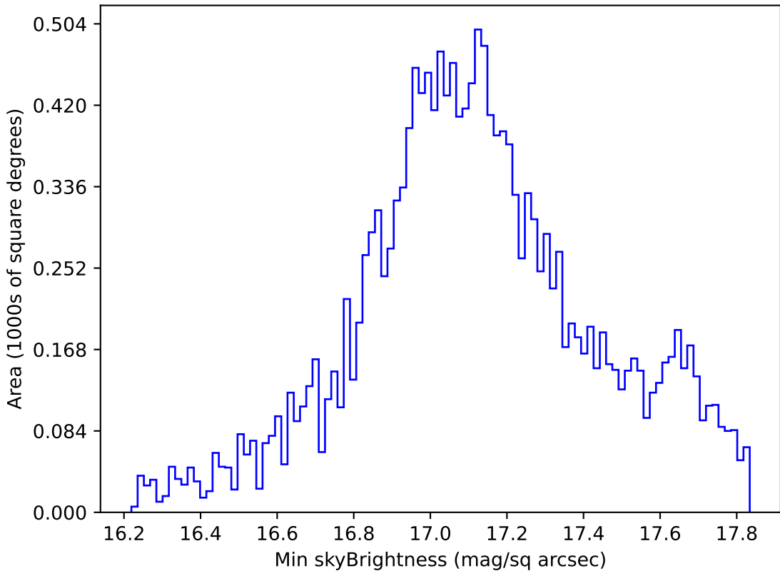
roll_pause_mjdp180_v3.4_10yrs WFD y band: Min skyBrightness
