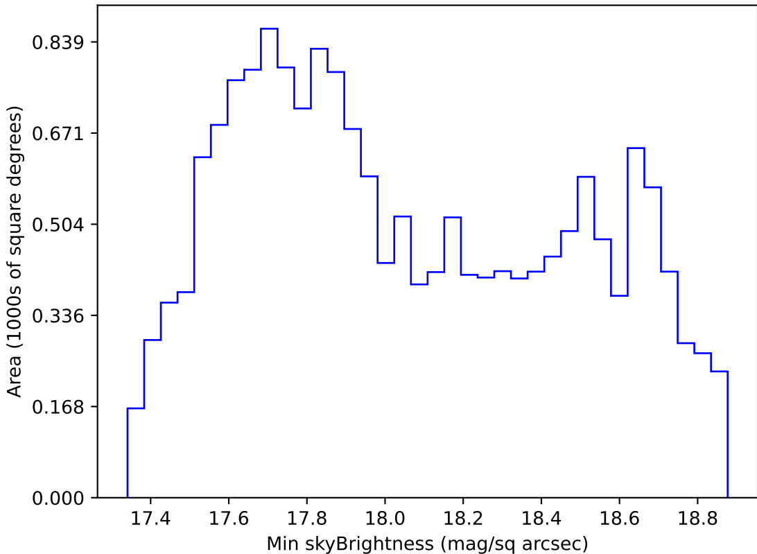
roll_pause_mjdp180_v3.4_10yrs WFD i band: Min skyBrightness
