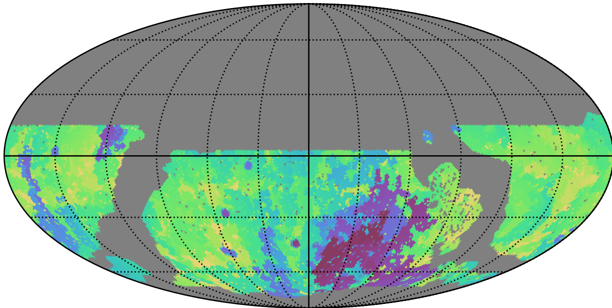
roll_pause_mjdp180_v3.4_10yrs WFD g band: Min skyBrightness
