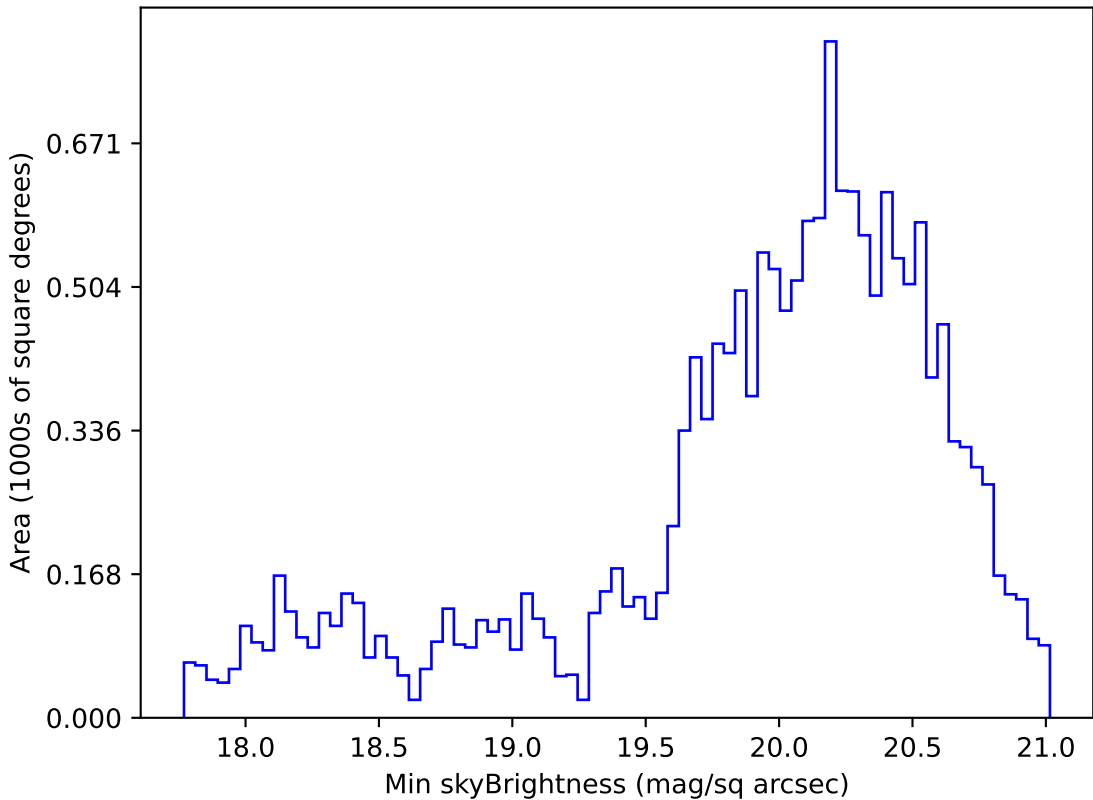
roll_pause_mjdp180_v3.4_10yrs WFD g band: Min skyBrightness
