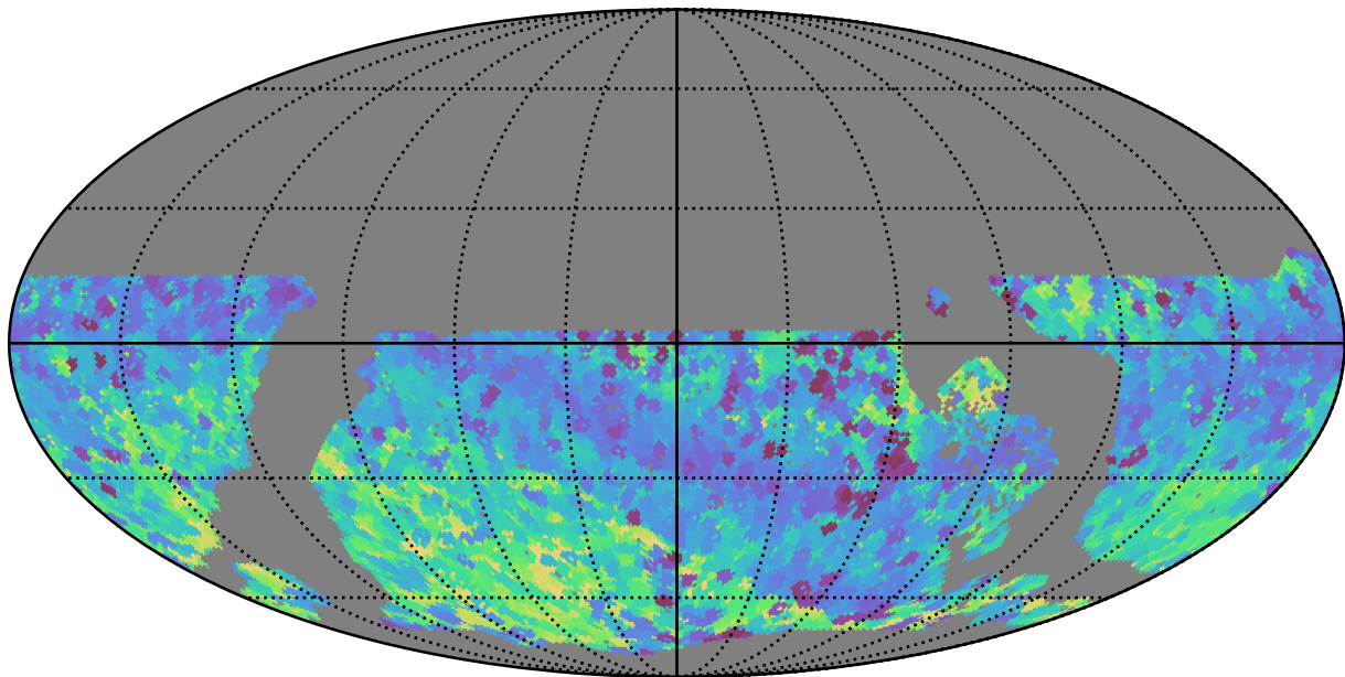
roll_pause_mjdp180_v3.4_10yrs WFD all bands: Min skyBrightness
