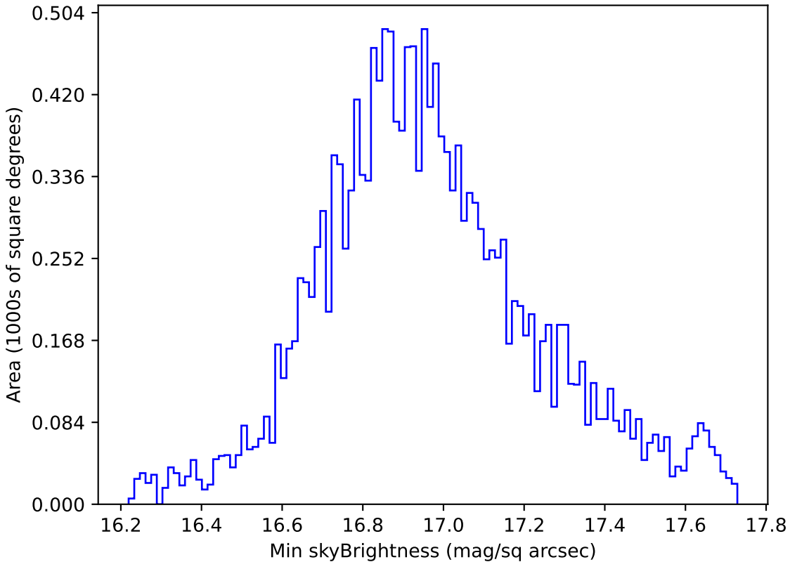
roll_pause_mjdp180_v3.4_10yrs WFD all bands: Min skyBrightness
