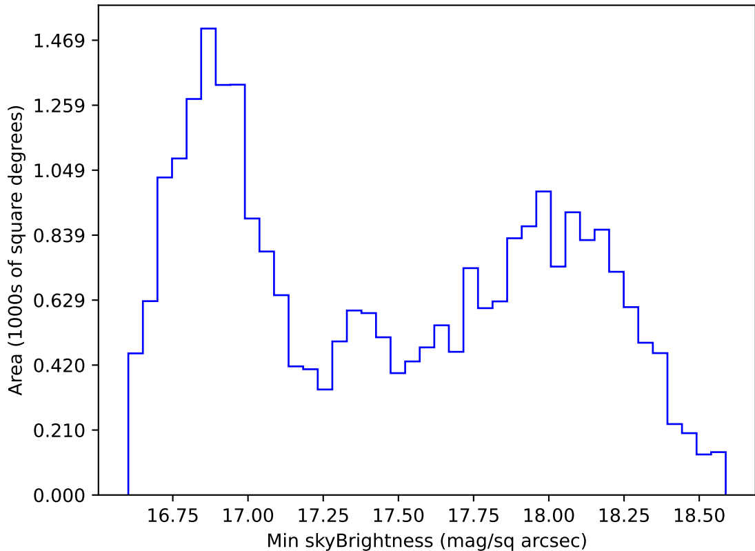
roll_pause_mjdp180_v3.4_10yrs All sky z band: Min skyBrightness
