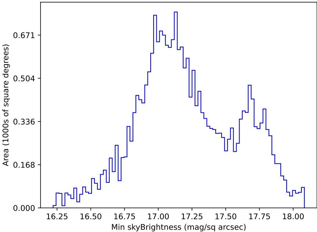
roll_pause_mjdp180_v3.4_10yrs All sky y band: Min skyBrightness
