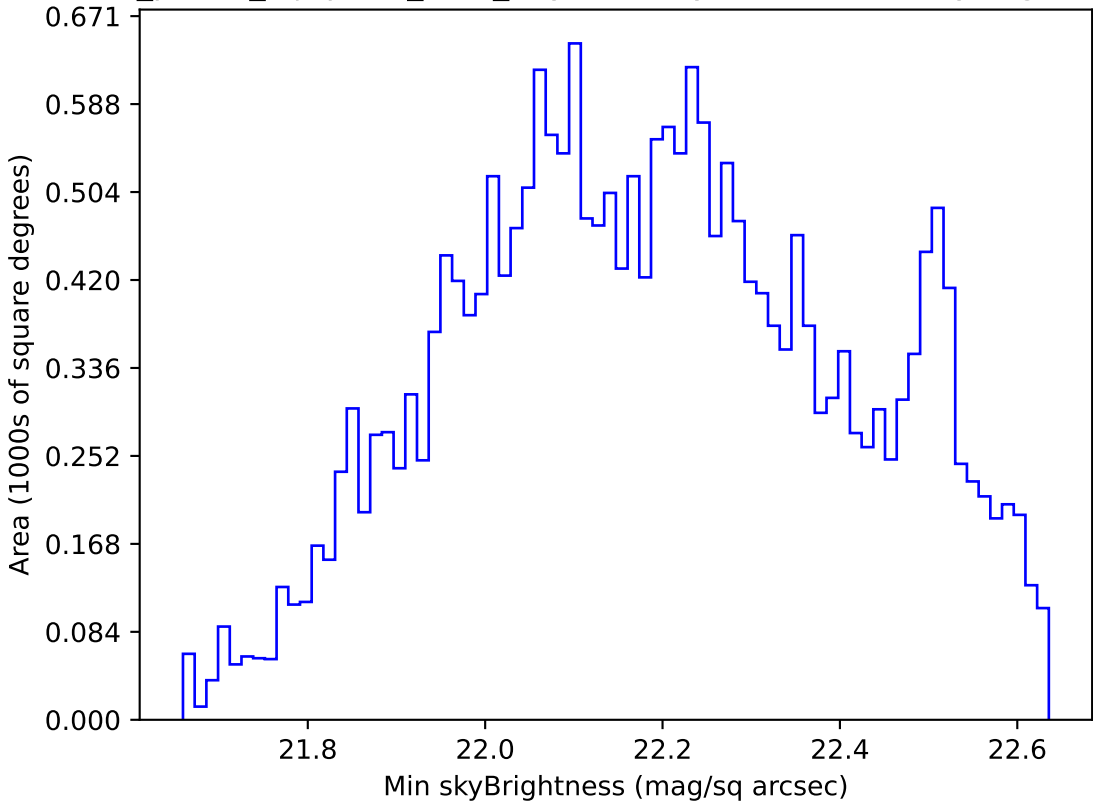
roll_pause_mjdp180_v3.4_10yrs All sky u band: Min skyBrightness
