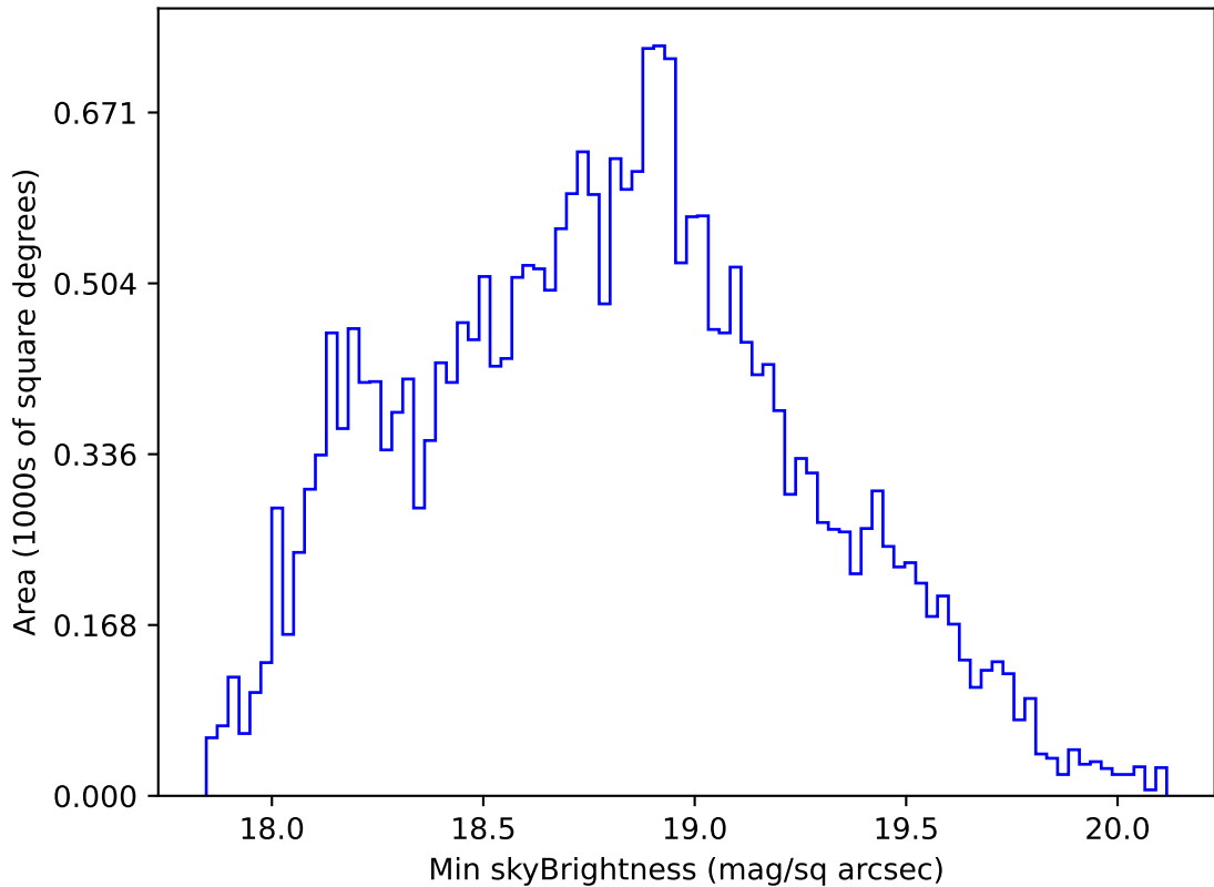
roll_pause_mjdp180_v3.4_10yrs All sky r band: Min skyBrightness
