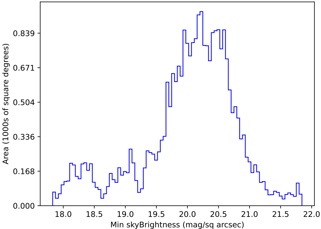
roll_pause_mjdp180_v3.4_10yrs All sky g band: Min skyBrightness
