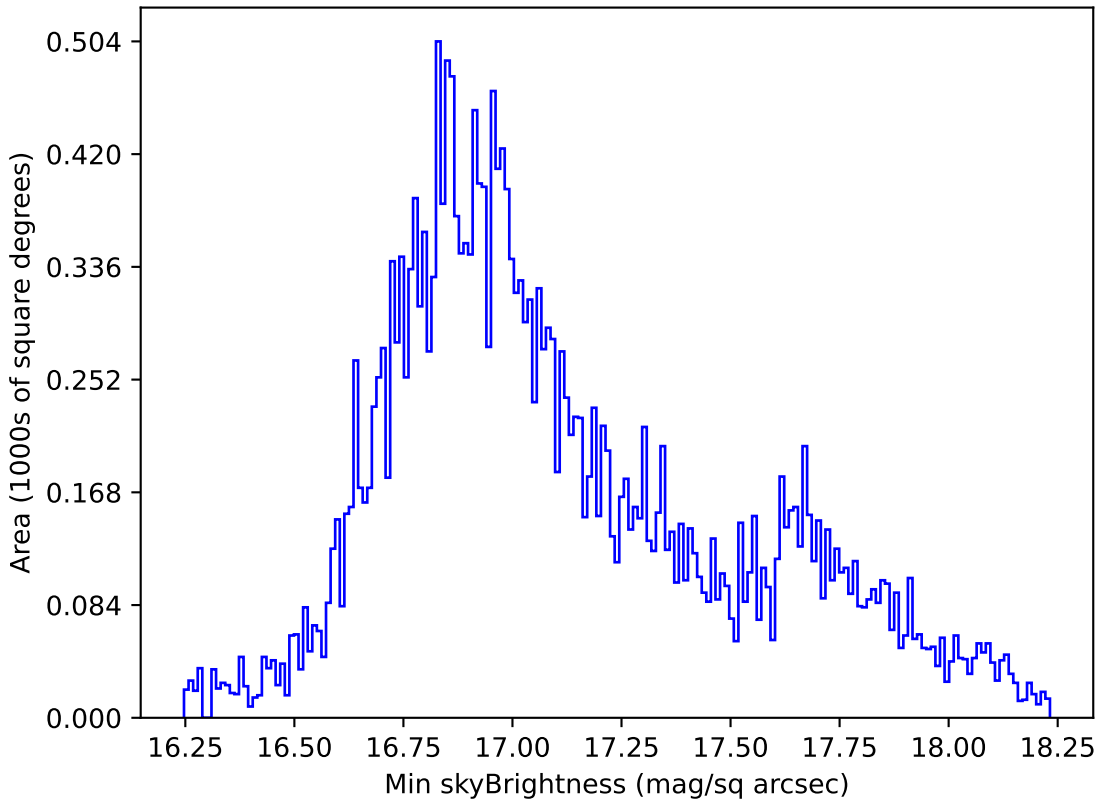
roll_pause_mjdp180_v3.4_10yrs All sky all bands: Min skyBrightness
