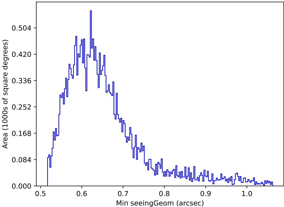
roll_pause_mjdp180_v3.4_10yrs Yr 1 z band: Min seeingGeom
