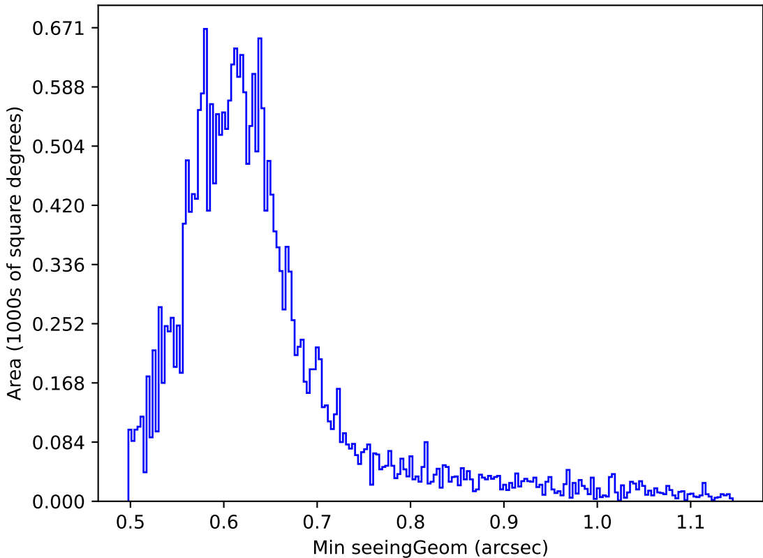
roll_pause_mjdp180_v3.4_10yrs Yr 1 r band: Min seeingGeom
