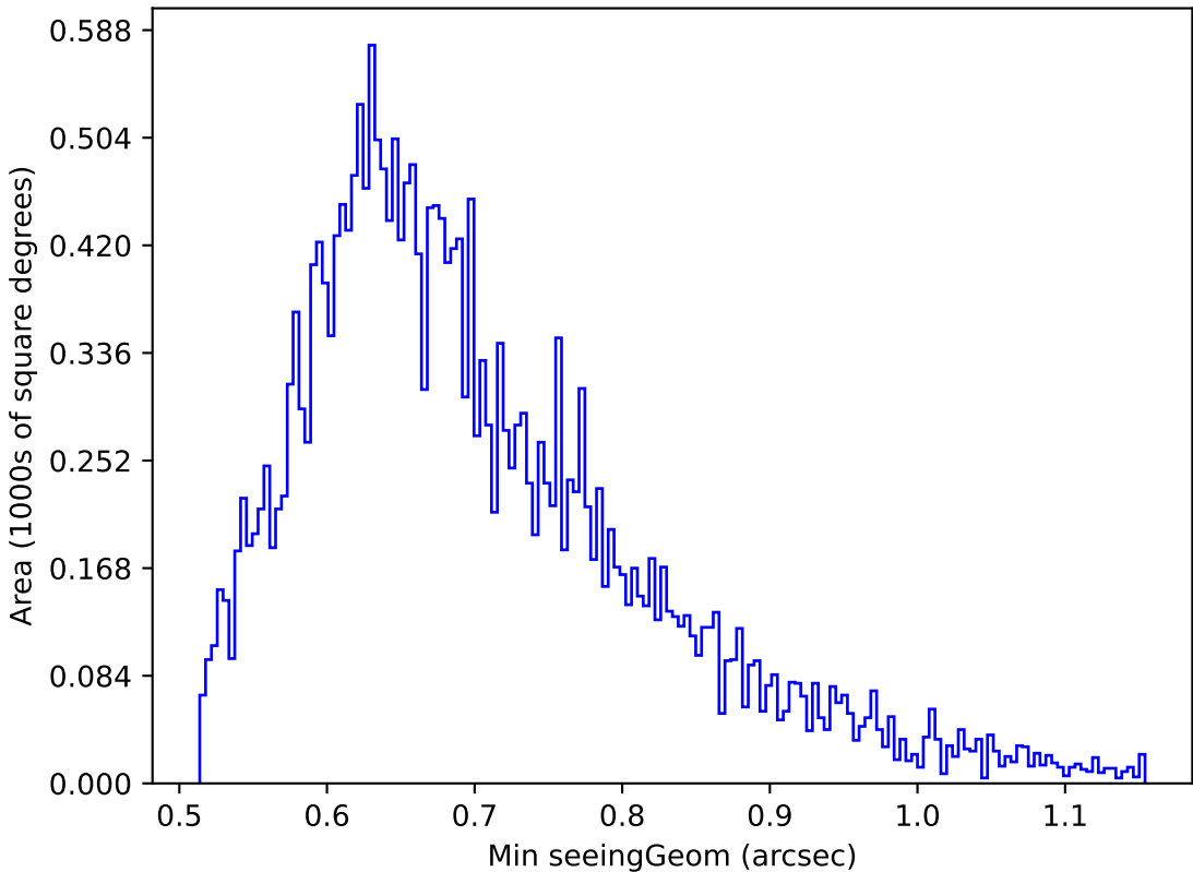
roll_pause_mjdp180_v3.4_10yrs Yr 1 g band: Min seeingGeom
