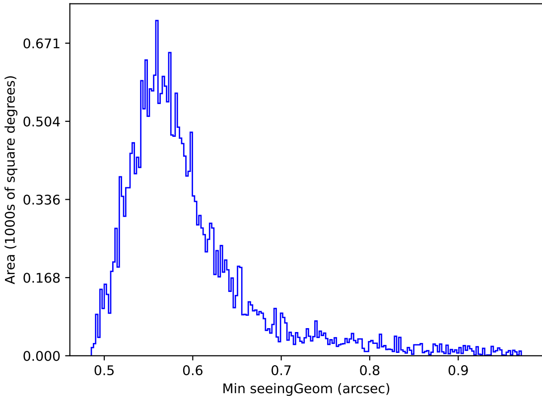
roll_pause_mjdp180_v3.4_10yrs Yr 1 all bands: Min seeingGeom
