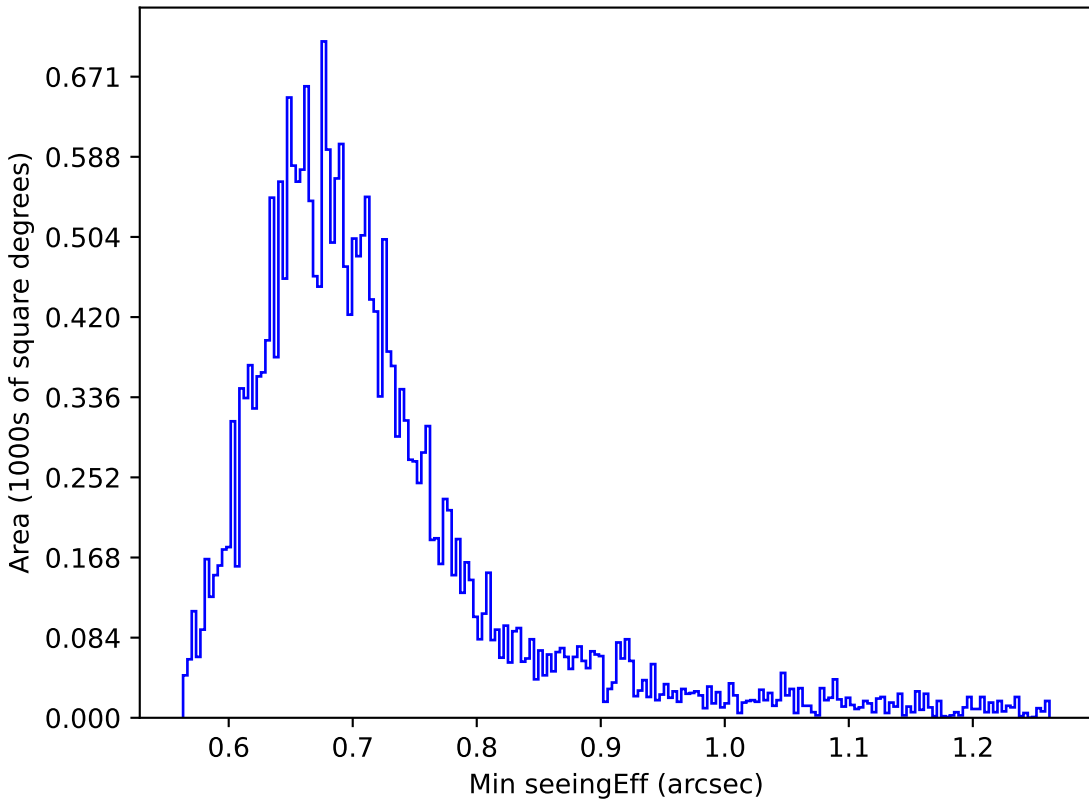
roll_pause_mjdp180_v3.4_10yrs Yr 1 i band: Min seeingEff
