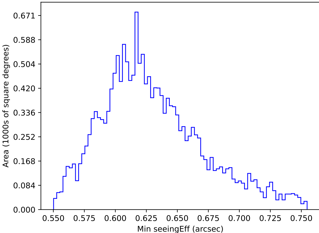
roll_pause_mjdp180_v3.4_10yrs WFD y band: Min seeingEff
