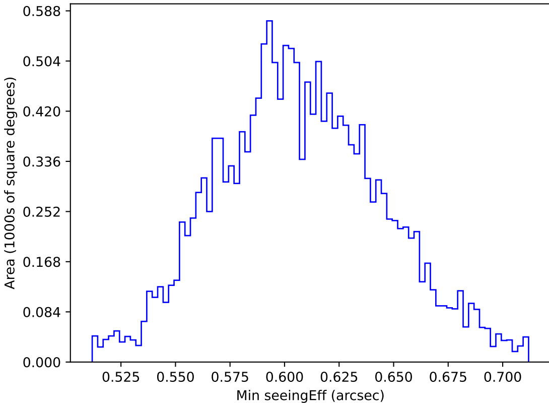
roll_pause_mjdp180_v3.4_10yrs WFD i band: Min seeingEff
