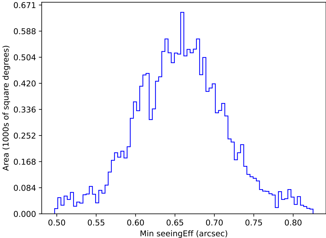
roll_pause_mjdp180_v3.4_10yrs WFD g band: Min seeingEff
