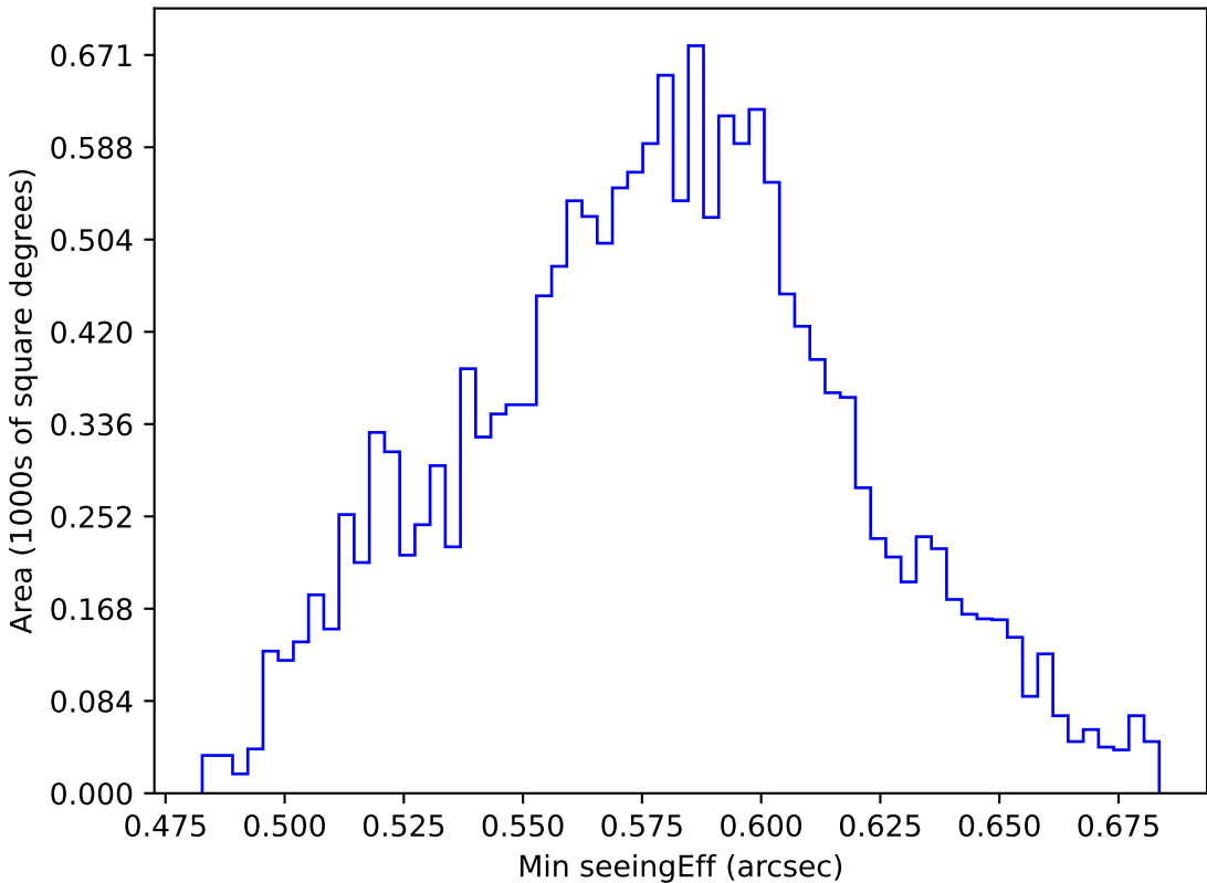
roll_pause_mjdp180_v3.4_10yrs WFD all bands: Min seeingEff
