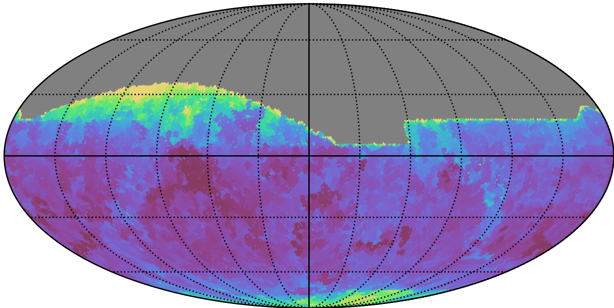
roll_pause_mjdp180_v3.4_10yrs All sky z band: Min seeingEff
