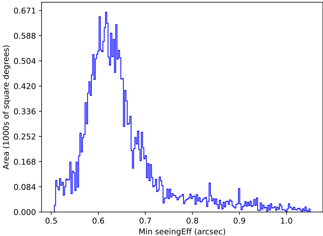
roll_pause_mjdp180_v3.4_10yrs All sky z band: Min seeingEff
